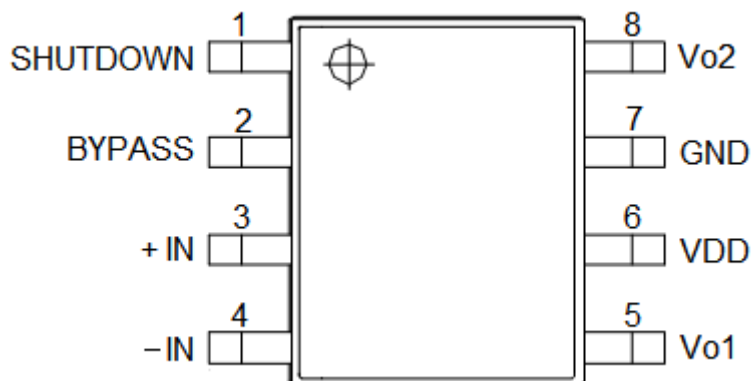
LY8896 8 Pin SOP (Top View)
