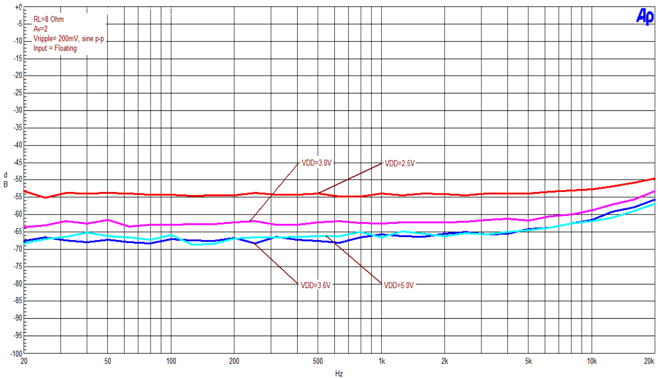
Figure 7 Power Supply Rejection Ratio (PSRR) at R_L=8\Omega , A_v=2 , Vripple = 200mVp-p, R_{IN} = Floating
