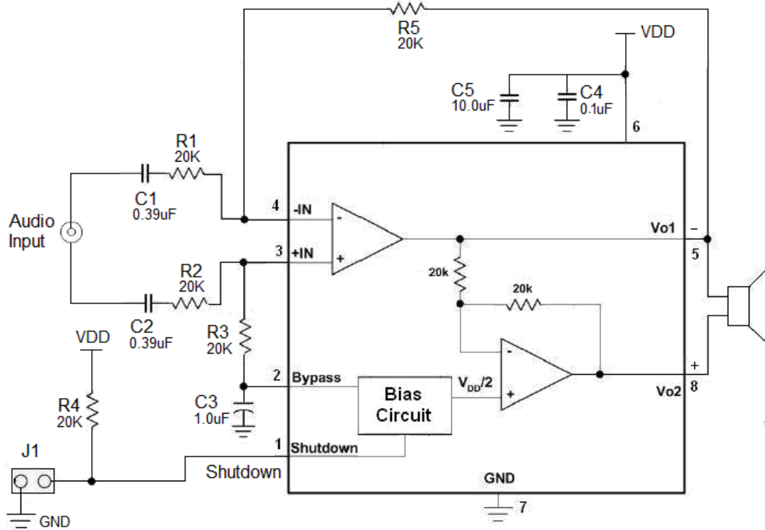
Figure 2. LY8896 application schematic with differential input
