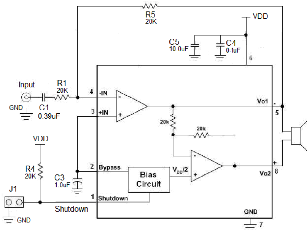
Figure 1. LY8896 application schematic with single-ended input
