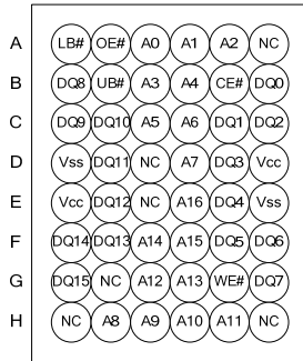
TFPGA(See through with Top View)
