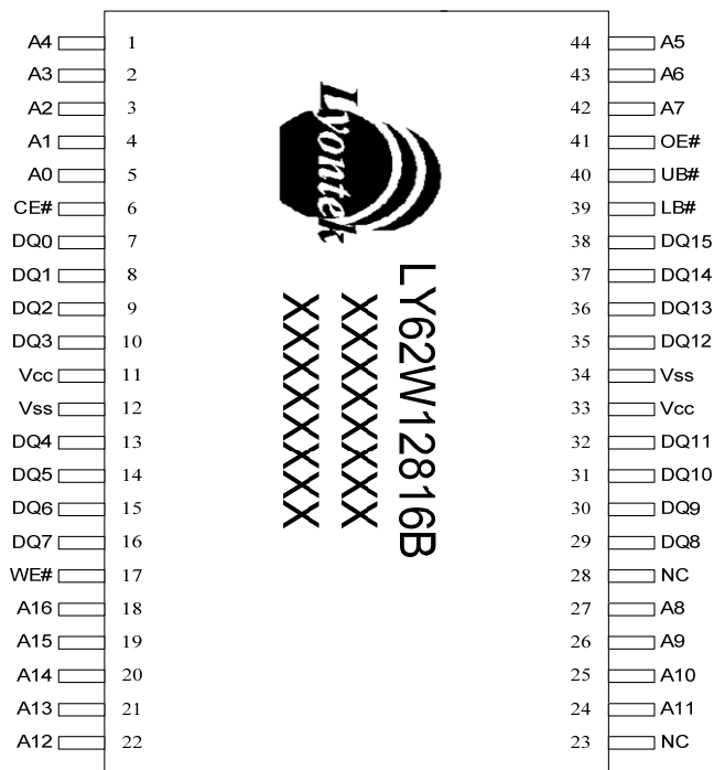
TSOP II
