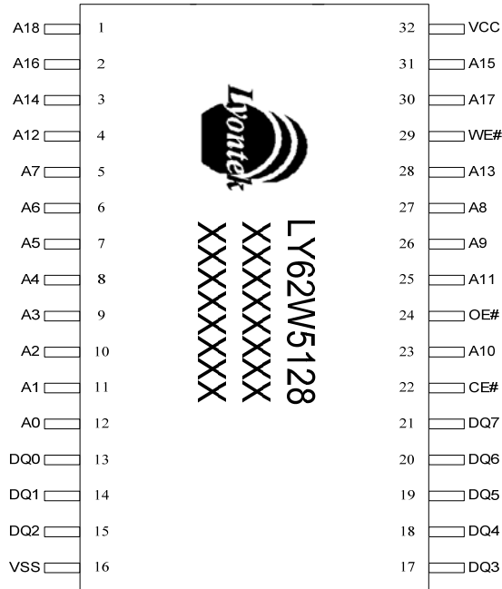
TSOP II
